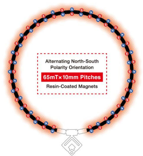
Magnet layout diagram
