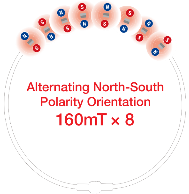
Magnet layout diagram
