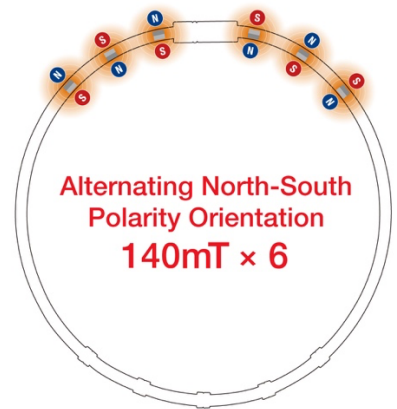
Magnet layout diagram
